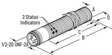
Figure 85. Micro QD Style
