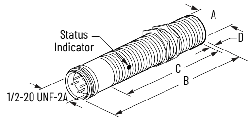
Figure 73. Micro QD Style
