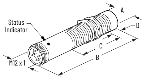
Figure 78. Micro QD Style
