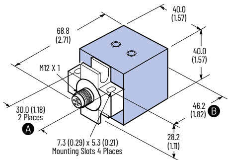
Figure 154. M12 Micro QD Style
