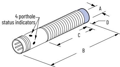
Figure 94. Pico QD Style
