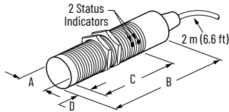
Figure 34. Cable Style
