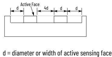
Figure 29. Flat Pack Style (Bul. 871F)
