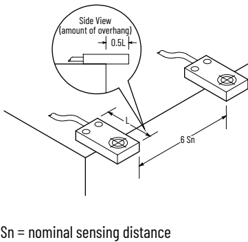
Figure 30. Miniature Flat Pack Style (Bul. 871FM)
