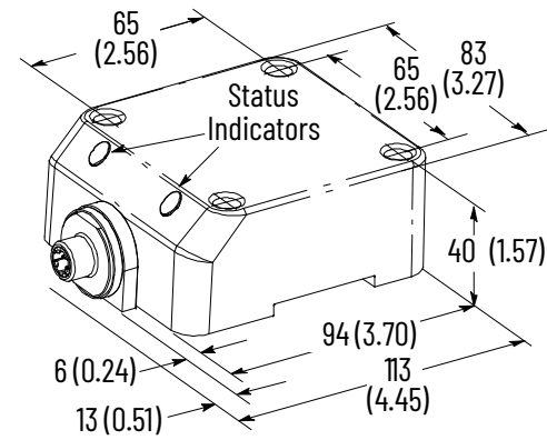
Figure 121. Conduit Style 1/2 in. NPT
