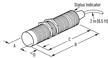
Figure 44. Cable Style
