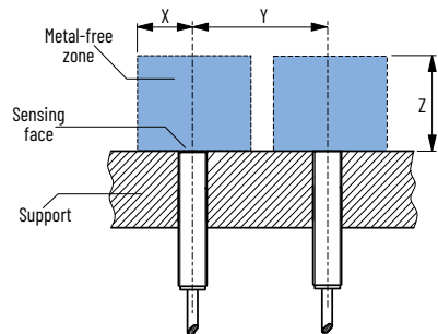
Figure 14. 871TM 3-wire DC Long Range Sensors Spacing
