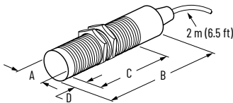
Figure 38. Cable Style
