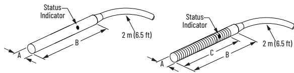
Figure 39. Cable Style
