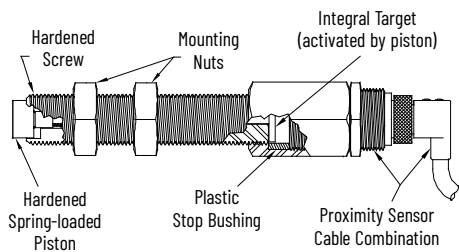
Figure 174. Banking Screw Adapter
