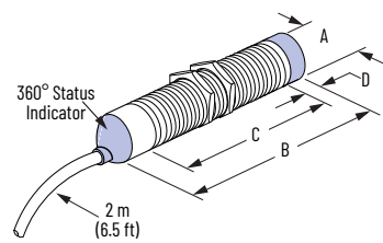
Figure 90. Cable Style
