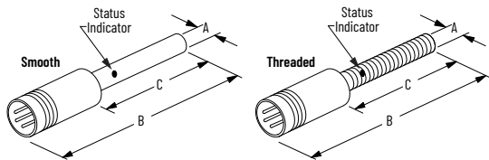
Figure 40. Pico QD Style
