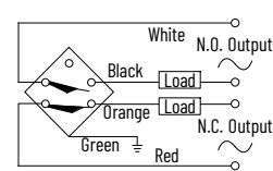
Figure 52. Cable Syle – Complementary N.O. or N.C.
