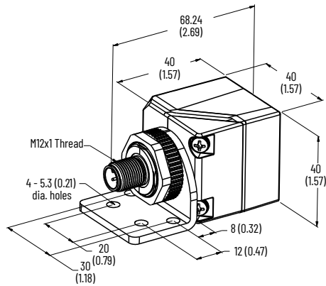
Figure 158. L Bracket
