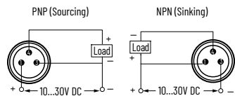
Figure 43. Pico QD and Pico with Lead Style – Normally Open
