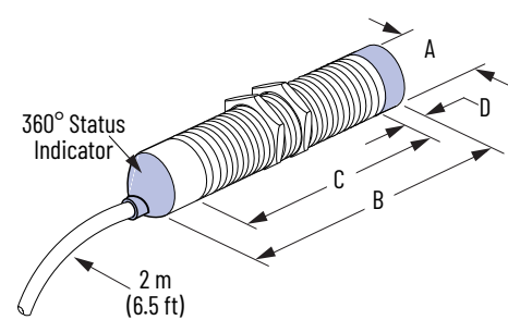
Figure 113. Cable Style
