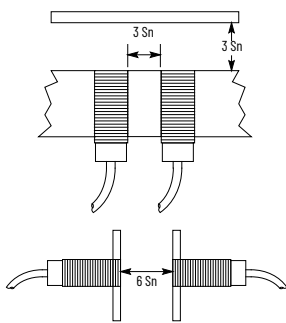
Figure 12. Tubular Style Extended Sensing (Bul. 872C)
