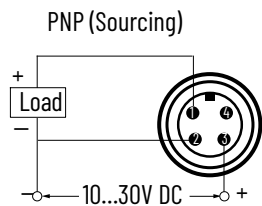
Figure 82. M12 Micro QD Style – N.O.
