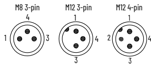
Figure 102. 8 mm, 12 mm, 18 mm, and 30 mm Pinouts
