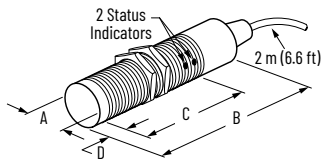
Figure 64. Cable Style
