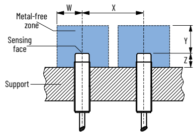
Figure 26. 871TM 3-wire DC Long Range Sensors Spacing
