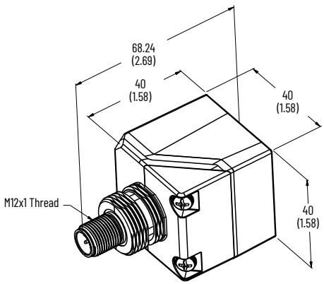
Figure 159. No Bracket
