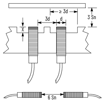
Figure 25. Tubular-style Long-range Sensing (Bul. 872C)
