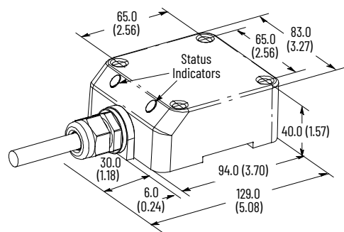
Figure 123. Cable Style
