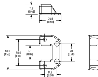
Figure 189. Dimensions in mm (in.)
