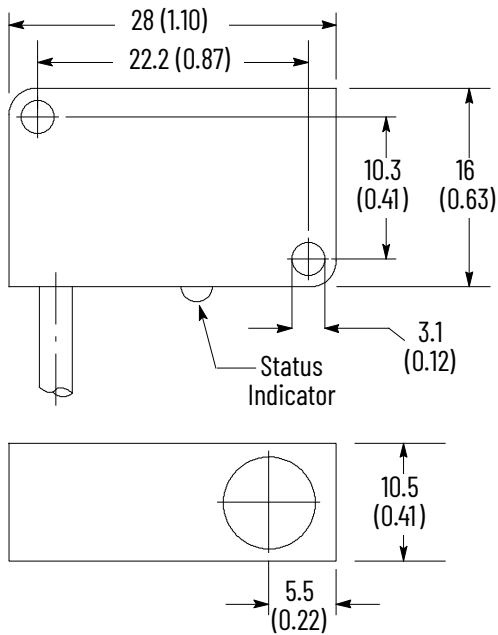
Figure 134. Cable and Pico QD Style (28 x 16 x 11 mm)
