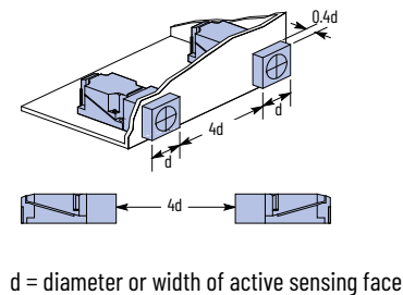
Figure 27. Limit Switch Style (Bul. 871L and 872L)
