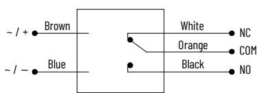
Figure 114. Cable Style
