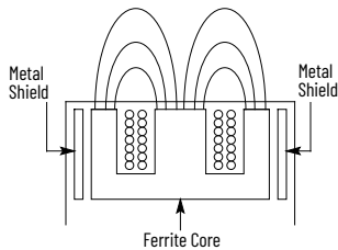
Figure 9. Shielded Sensor
