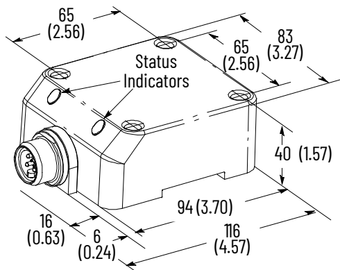
Figure 125. Micro QD Style
