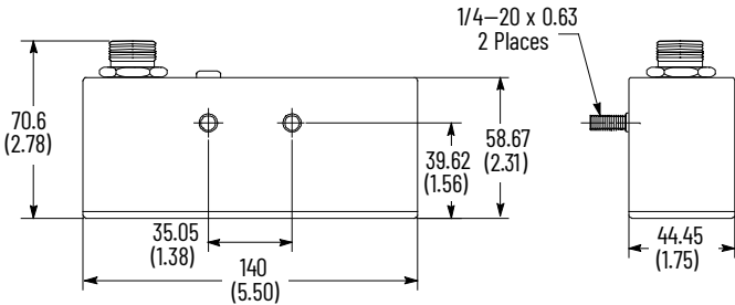
Figure 150. Mini and M12 Micro QD Style
