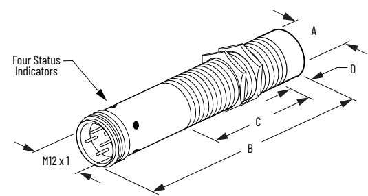
Figure 93. M12 Micro Style
