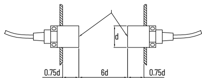
Figure 33. Spacing Between Opposing Sensors
