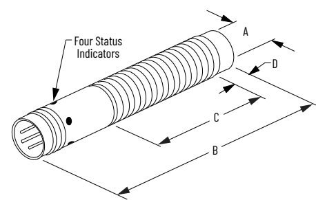
Figure 62. M8 Pico Style
