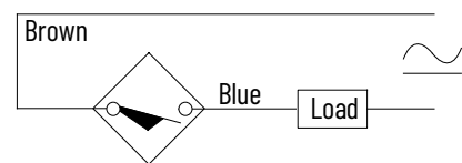
Figure 75. Cable Style – N.O.
