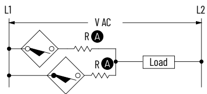
Figure 8. Wiring Diagram for Parallel Connected AC Sensors
