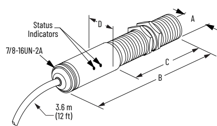
Figure 50. Cable Style
