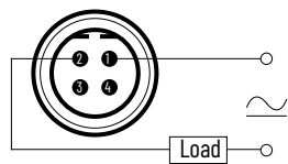
Figure 74. EAC M12 Micro QD Style – N.O.
