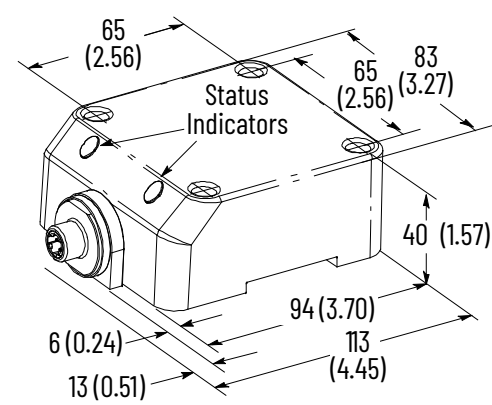
Figure 130. Micro QD Style
