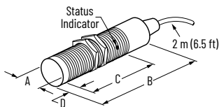
Figure 71. Cable Style
