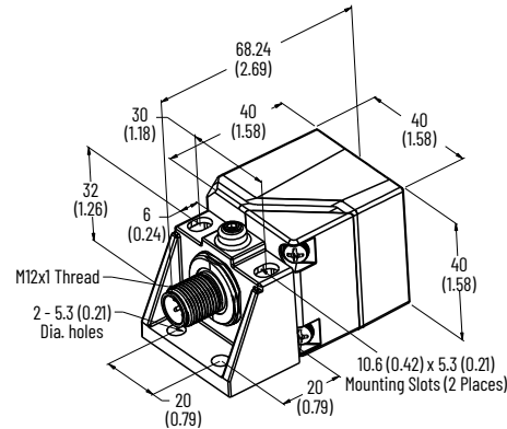
Figure 157. Zinc Bracket
