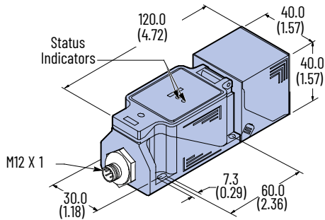
Figure 139. M12 Micro QD Style
