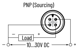
Figure 89. M12 Micro QD Style – N.O.
