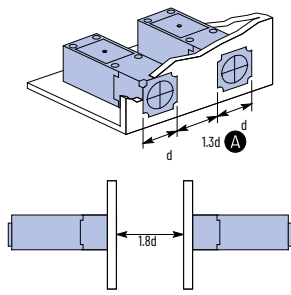
Figure 16. Limit Switch Style (Bul. 802PR)
