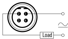
Figure 67. EAC M12 Micro QD Style – N.O.
