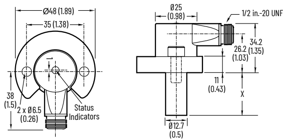
Figure 165. M12 Micro QD Style
