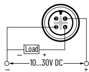
Figure 47. M12 Micro QD Style – Normally Open, PNP (Sourcing)
