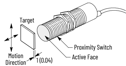
Figure 1. Standard Target [mm (in.)]
