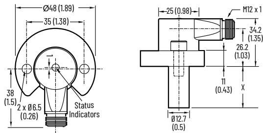
Figure 168. M12 Micro QD Style
