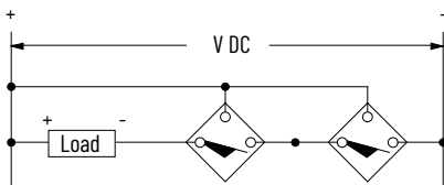
Figure 5. Wiring Diagram for Series Connected Current Source Sensors (PNP)
