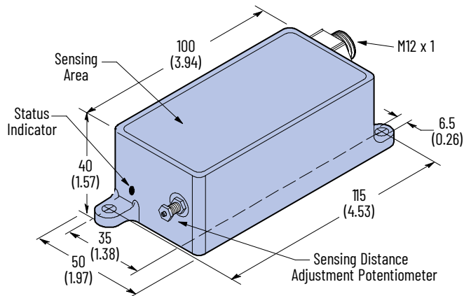
Figure 118. Micro QD Style
