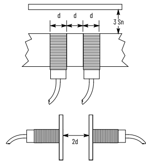
Figure 11. Tubular Style
