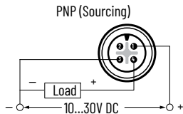
Figure 82. M12 Micro QD Style – N.O.
