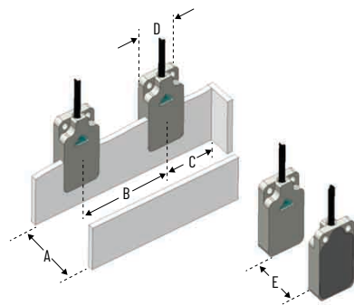
Figure 19. 871FM Miniature Metal Flat Pack Sensors Spacing
