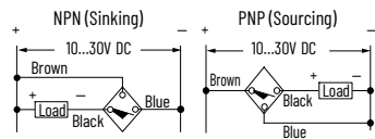
Figure 43. Pico QD and Pico with Lead Style – Normally Open
