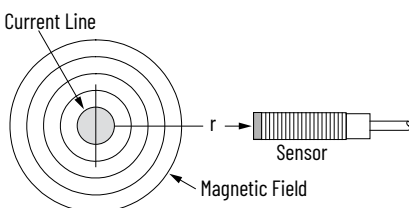
Figure 2. Perpendicular Mounting to the Current Line
