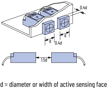
Figure 28. Limit Switch Style (Bul. 802PR)
