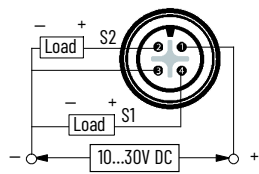
Figure 170. Normally Open – PNP (Sourcing)
