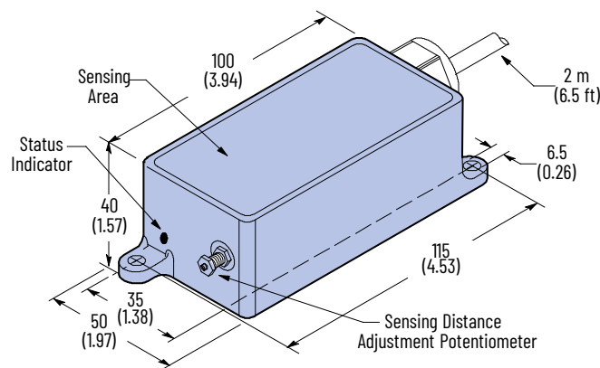
Figure 117. Cable Style
