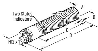
Figure 88. M12 Micro QD Style
