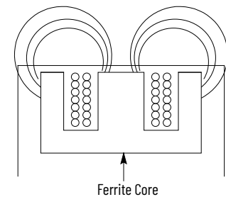
Figure 10. Unshielded Sensor
