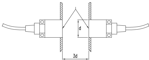
Figure 22. Spacing Between Opposing Sensors
