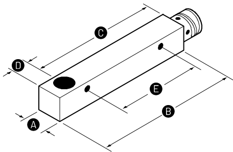
Figure 136. M8 Square 3-pin Pico
