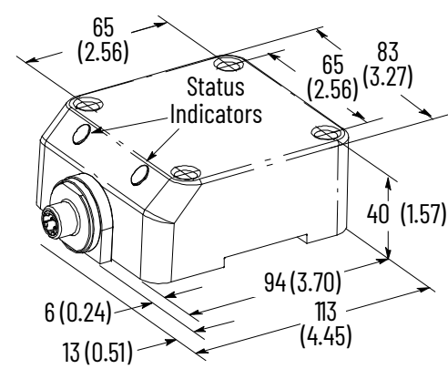
Figure 129. M12 Micro QD Style
