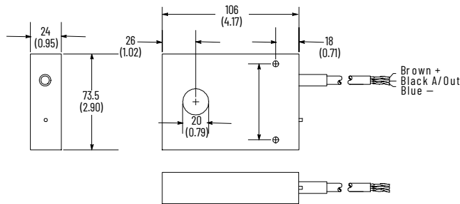
Figure 172. Cable Style
