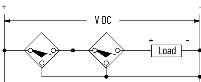
Figure 5. Wiring Diagram for Series Connected Current Source Sensors (PNP)
