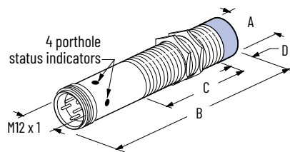
Figure 95. M12 Micro QD Style
