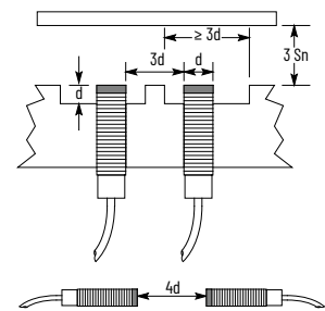
Figure 23. Tubular Style
