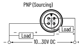
Figure 169. M12 Micro QD Style – Normally Open
