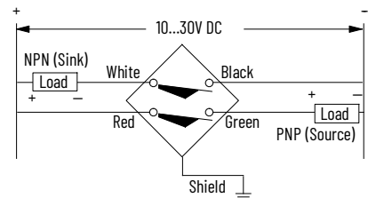
Figure 151. Cable Style
