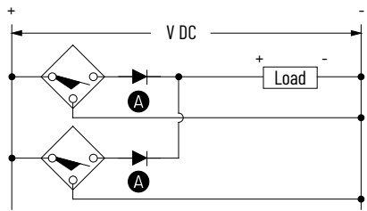
Figure 7. Wiring Diagram for Parallel Connected Current Source Sensors (PNP)
