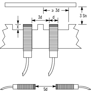
Figure 13. Tubular-style Long-range Sensing (Bul. 872C)
