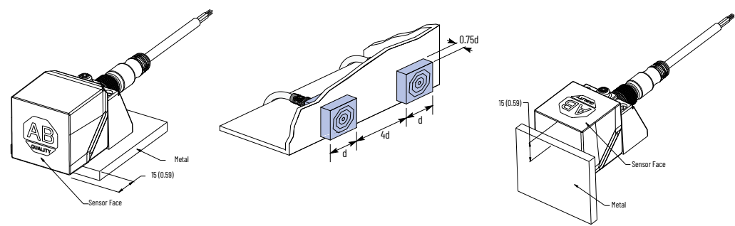
Figure 32. 871P VersaCube Sensor (4-wire [mm (in.)])
