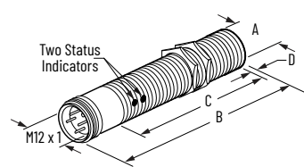
Figure 61. M12 Micro Style
