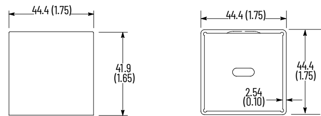
Figure 191. Cat. No. 871A-KCT40-F
