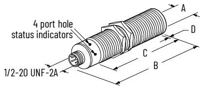
Figure 107. Micro QD Style
