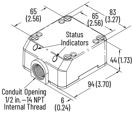
Figure 126. Conduit Style 1/2 in. NPT
