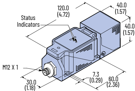
Figure 142. M12 Micro QD Style
