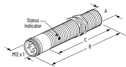
Figure 80. M12 Micro QD Style
