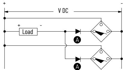
Figure 6. Wiring Diagram for Parallel Connected Current Sink Sensors (NPN)
