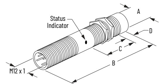
Figure 70. EAC M12 Micro QD Style
