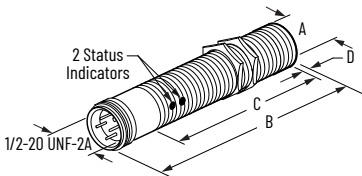
Figure 36. AC Micro QD Style
