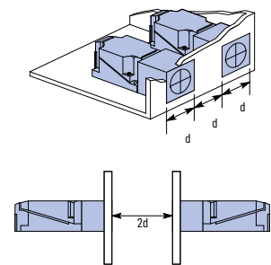
Figure 15. Limit Switch Style (Bul. 871L/872L)
