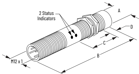
Figure 63. EAC M12 Micro QD Style
