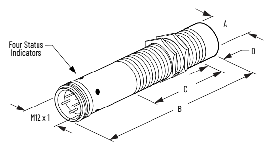
Figure 54. Micro QD Style
