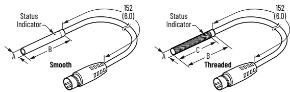
Figure 41. Pico with Lead Style [mm (in.)]
