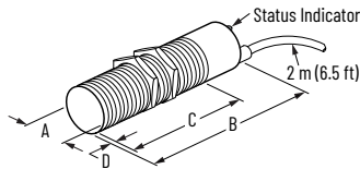
Figure 108. Cable Style
