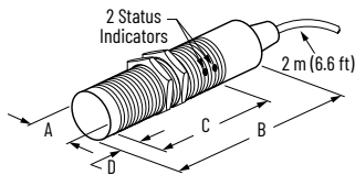
Figure 83. Cable Style
