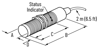
Figure 58. Cable Style
