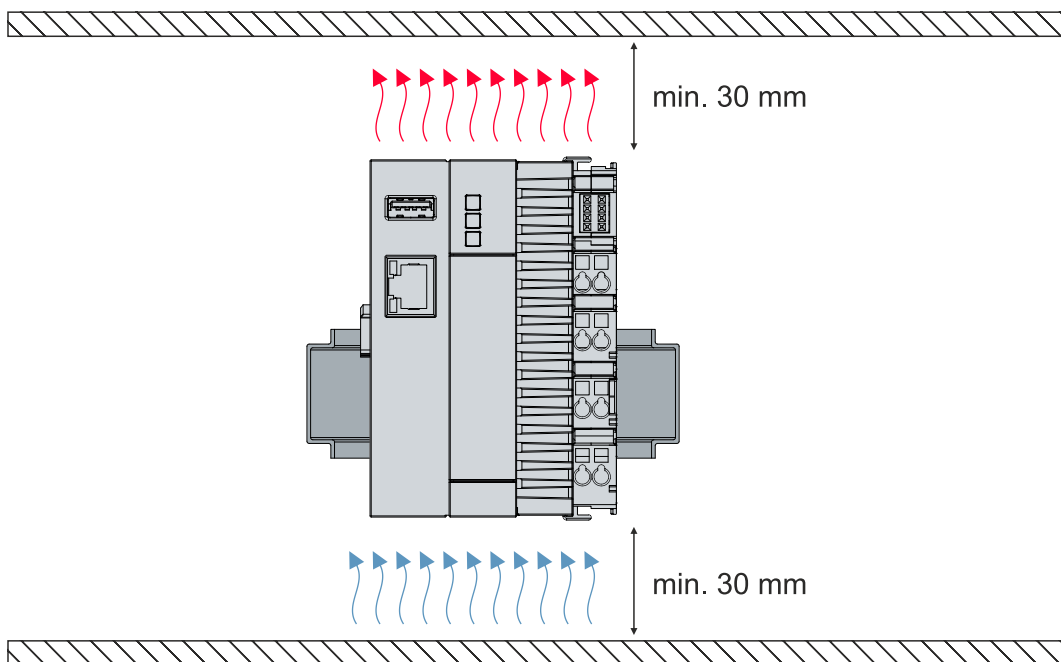
Fig. 6: CX82xx Embedded PC, approved installation position.
