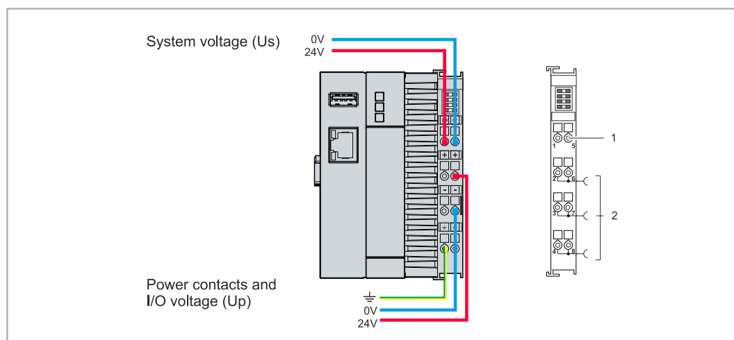
Fig. 10: Connections for system voltage (Us) and power contacts (Up).
