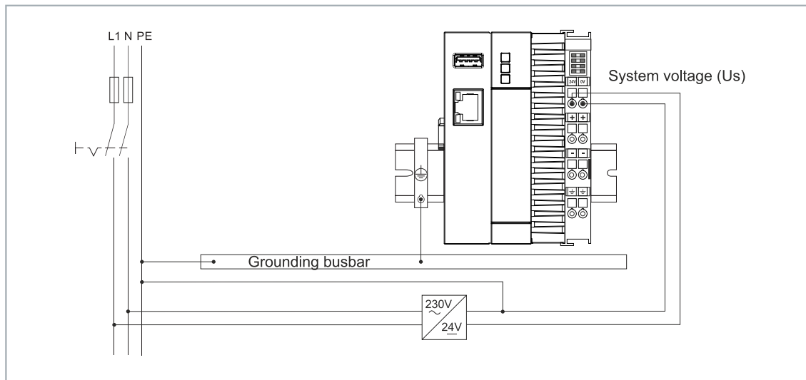
Fig. 11: Connection example with a CX8200.
