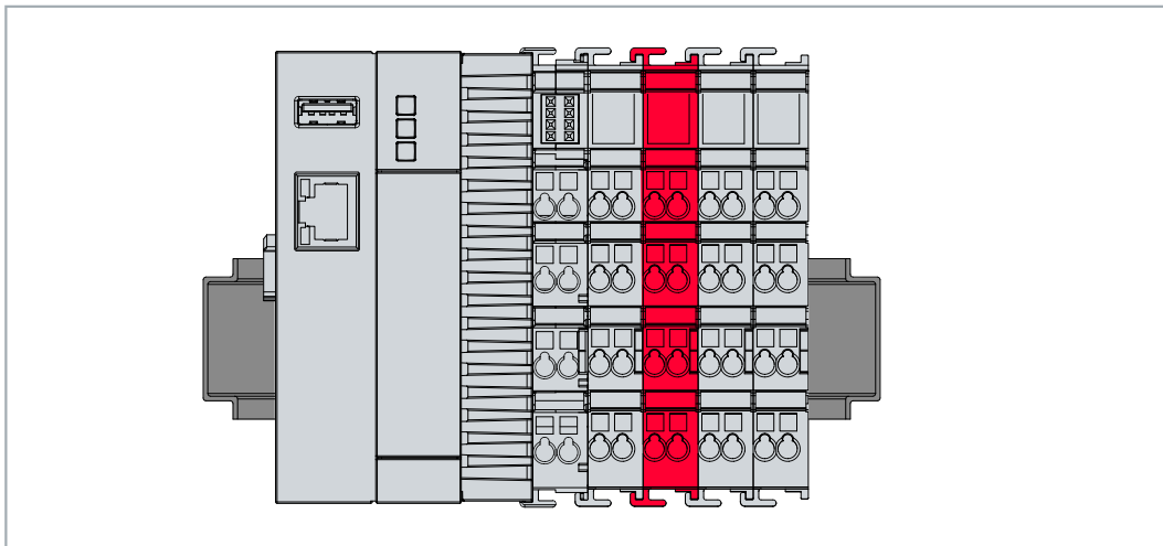
Fig. 9: Passive EtherCAT Terminals, permissible installation.
