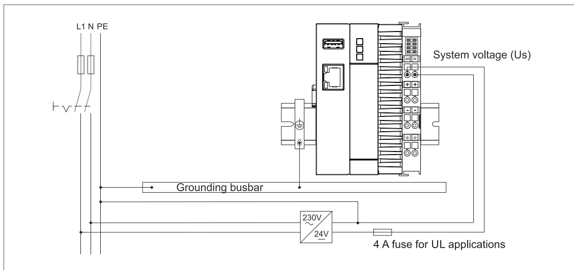
Fig. 13: Connection example for areas with special UL requirements.
