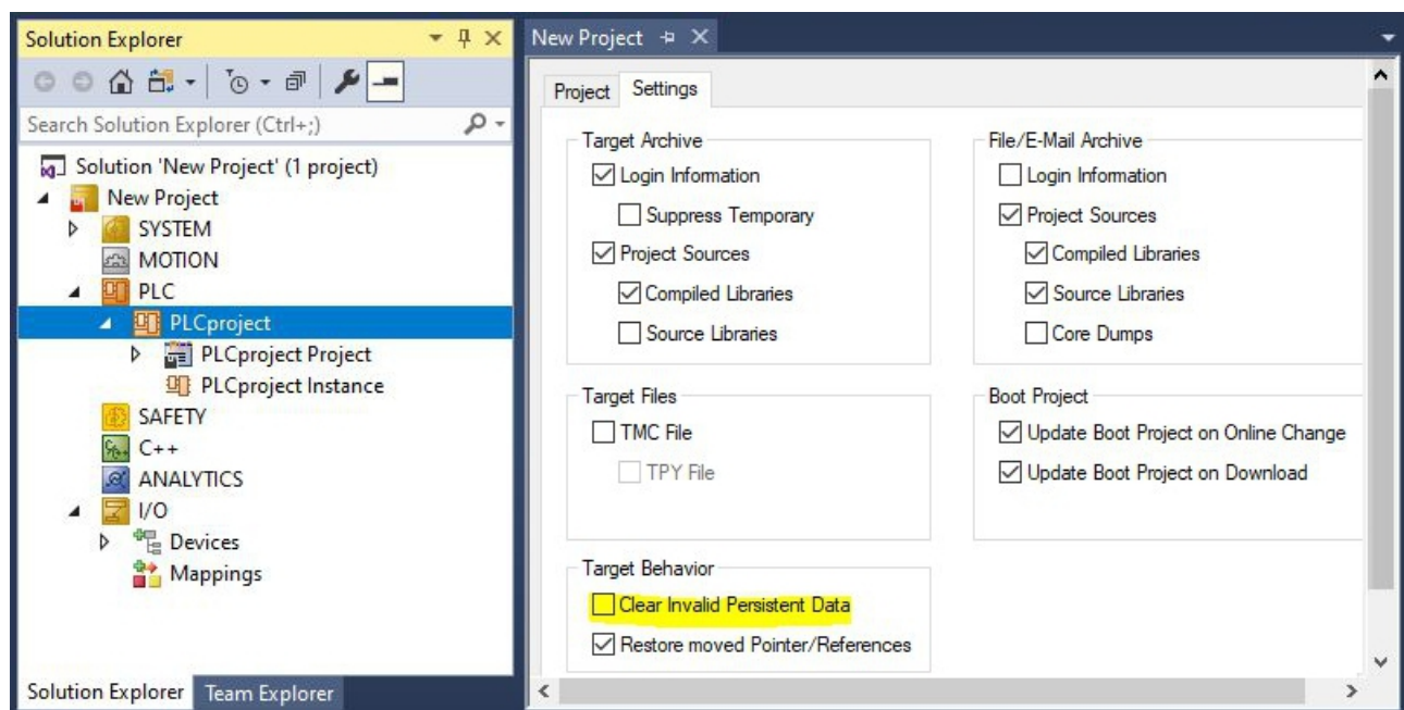
Fig. 15: Load a backup of the persistent data. Settings in TwinCAT 3.
