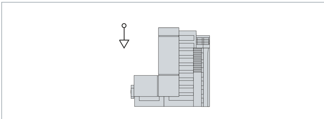
Fig. 7: CX82xx Embedded PC, installation position with limited temperature range
