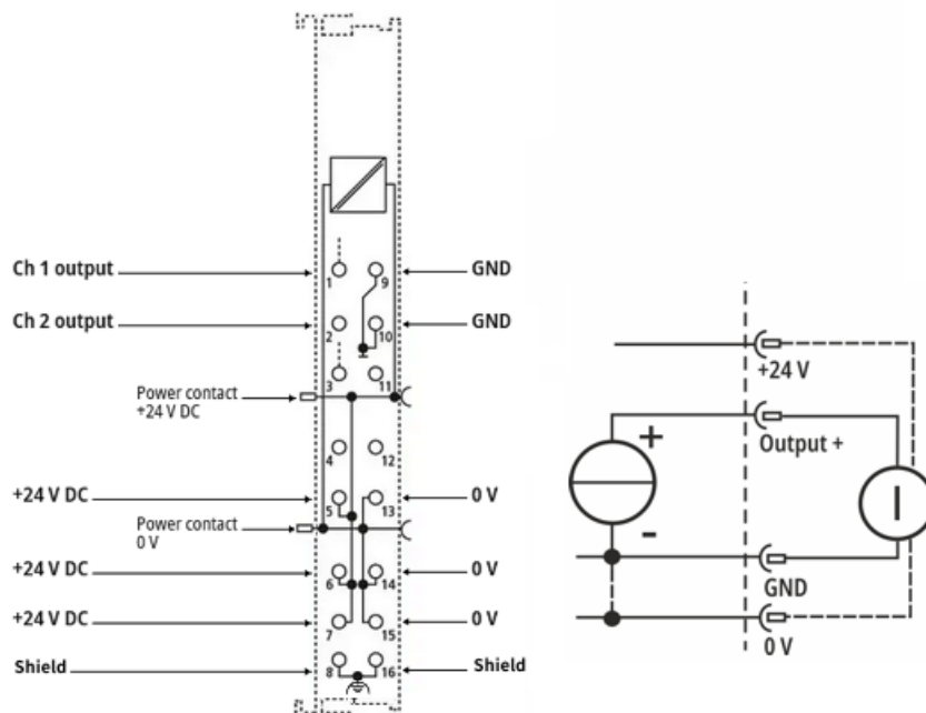
Fig. 3: Connection example ED4072, current output, 2-/4-wire
