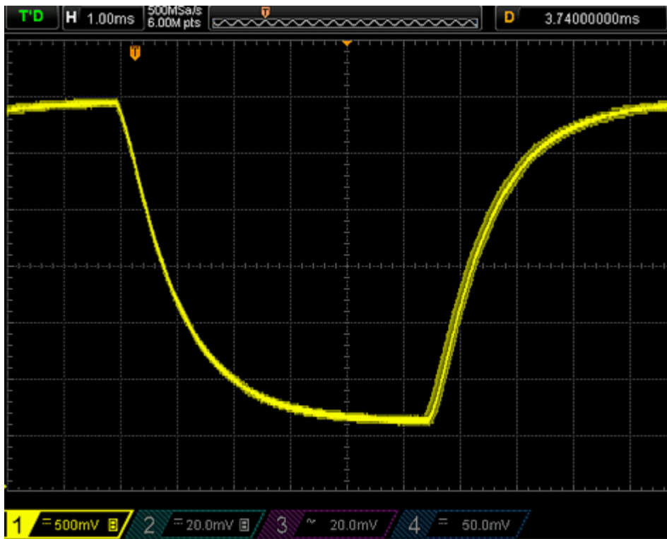
Fig. 27: EL4078 with 500 µs EtherCAT cycle time, output jitter \pm 0.5 cycle according to theory
