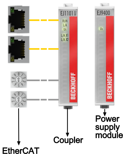
Fig. 16: E-bus power supply with EJ1100 or EJ1101-0022 + EJ940x
