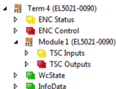
Fig. 32: TwinSAFE SC component process data, example EL5021-0090
