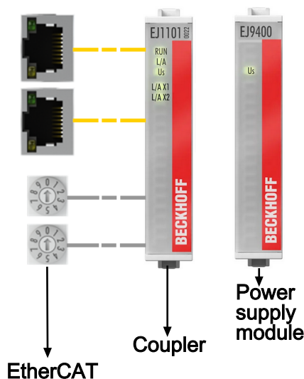
Fig. 13: E-bus power supply with EJ1100 or EJ1101-0022 + EJ940x
