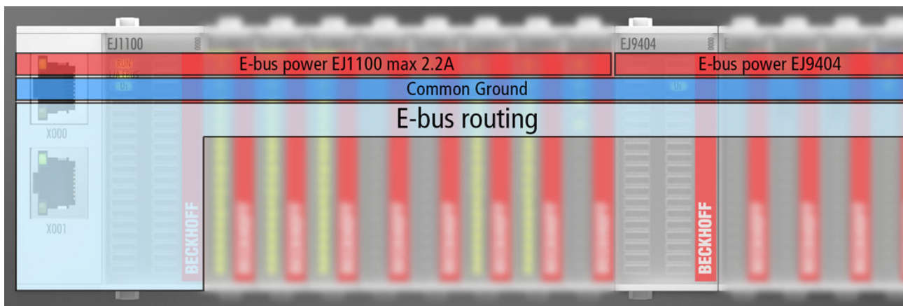
Fig. 11: Using the EJ9404 power supply plug-in module for E-bus refresh
