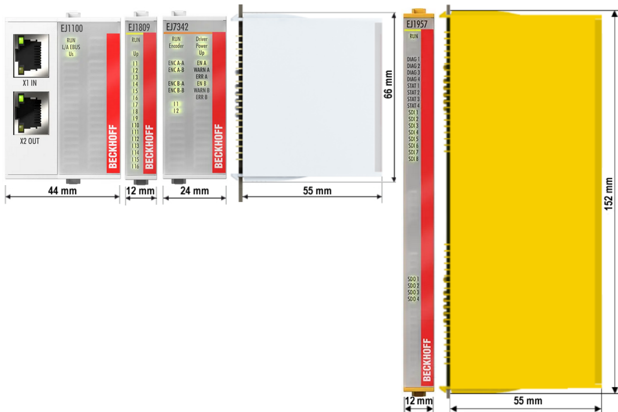
Fig. 15: EJxxxx - Dimensions
