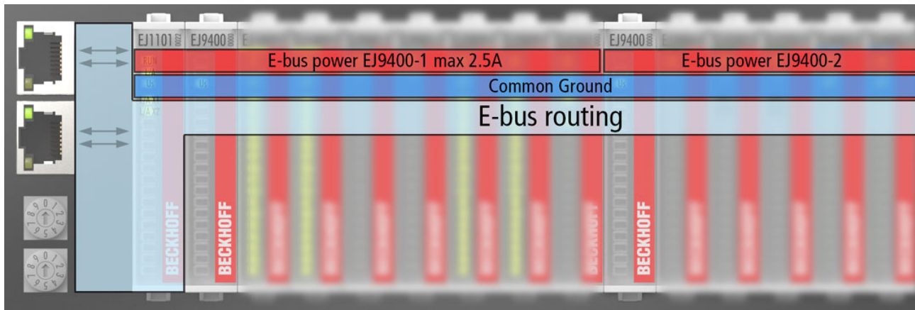
Fig. 10: Using the EJ9400 power supply plug-in module for E-bus refresh
