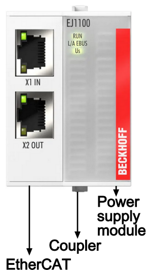
Fig. 13: E-bus power supply with EJ1100 or EJ1101-0022 + EJ940x
