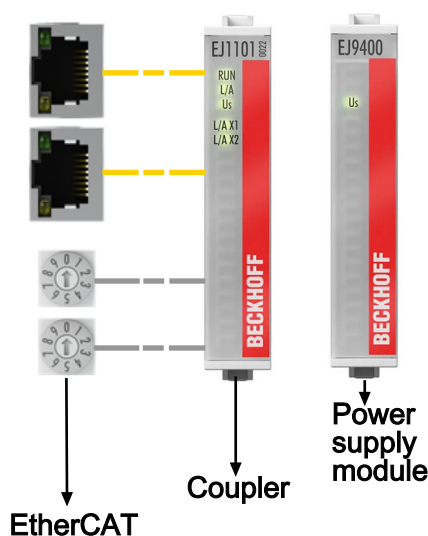
Fig. 13: E-bus power supply with EJ1100 or EJ1101-0022 + EJ940x
