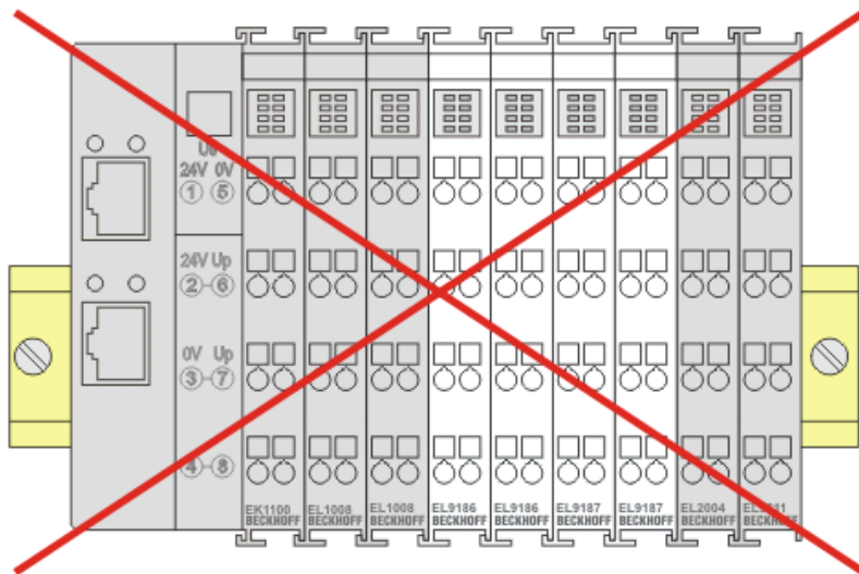
Fig. 8: Incorrect positioning
