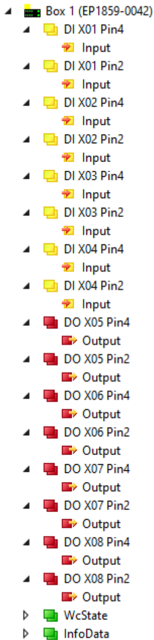
Fig. 21: EP1859-0042 - Process image
