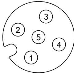
Fig. 25: M12 socket
