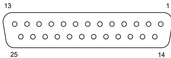
Fig. 33: D-sub socket, 25-pin
