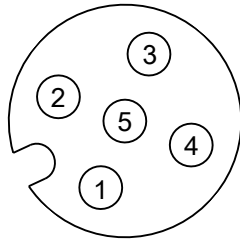
Fig. 36: M12 socket
