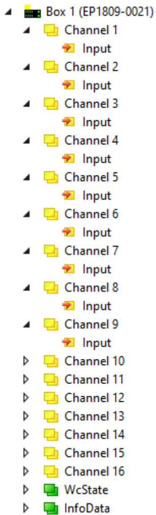
Fig. 6: EP1809-0021, Process image
