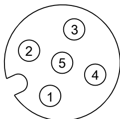
Fig. 30: M12 socket
