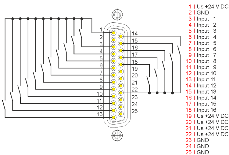
Fig. 34: Digital inputs D-sub, connection examples
