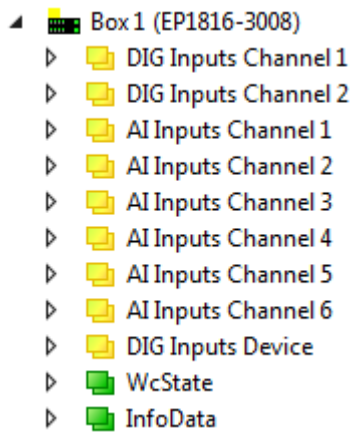
Fig. 16: EP1816-3008 Process image
