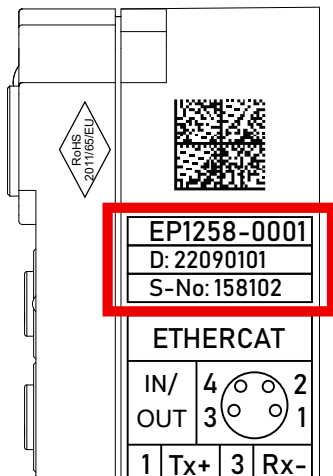
Fig. 3: EP1258-00001 IP67 EtherCAT Box with batch number/DateCode 22090101 and unique serial number 158102
