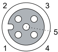
Fig. 20: M12 socket
