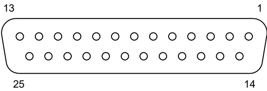
Fig. 12: D-sub socket, 25-pin
