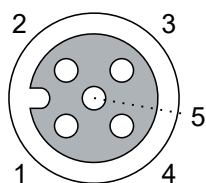
Fig. 18: M12 socket, 5-pin
