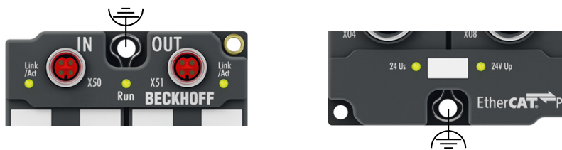
Fig. 7: Connection for functional earth (FE)
