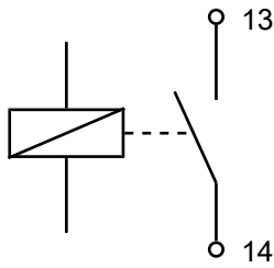
Fig. 19: Relay connections
