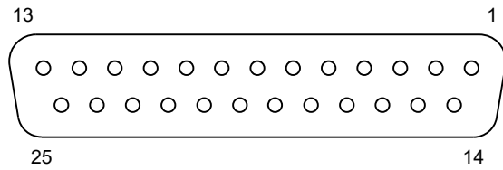
Fig. 16: D-sub socket, 25-pin
