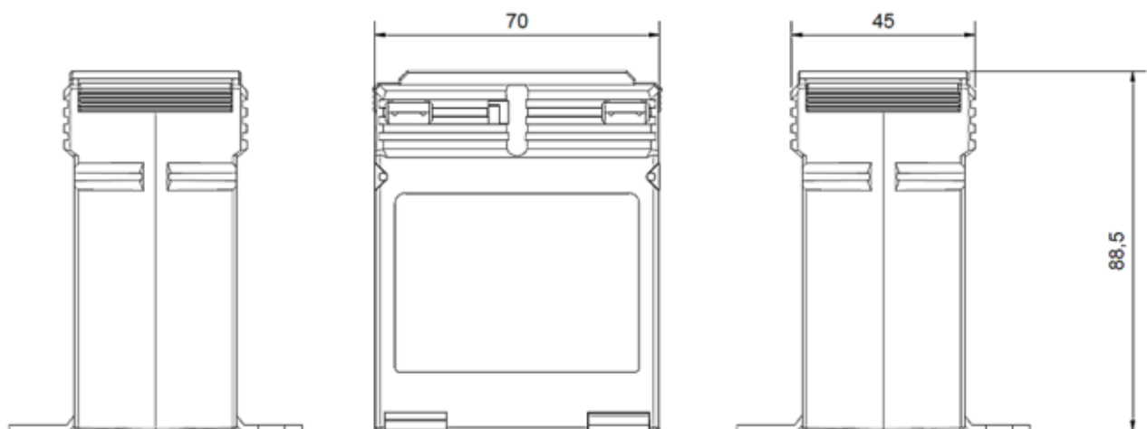
Fig. 18: Right side view, front view, left side view; all dimensions in mm
