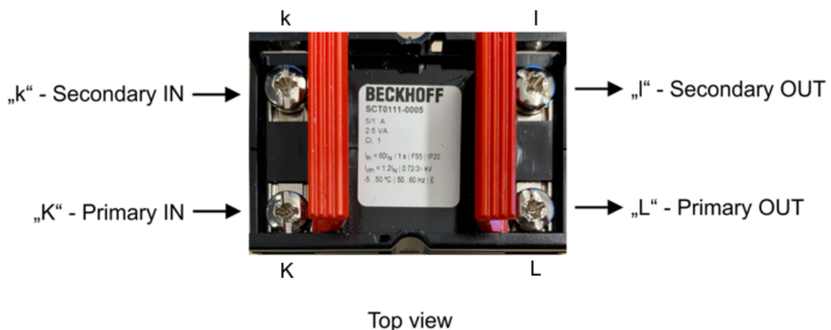
Fig. 19: SCT0xxx connections
