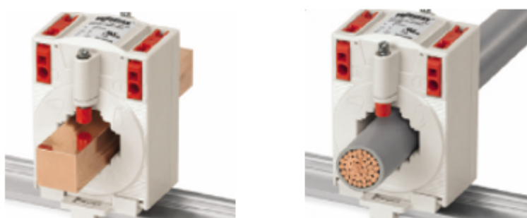
Fig. 32: Mounting on copper bar or round conductor
