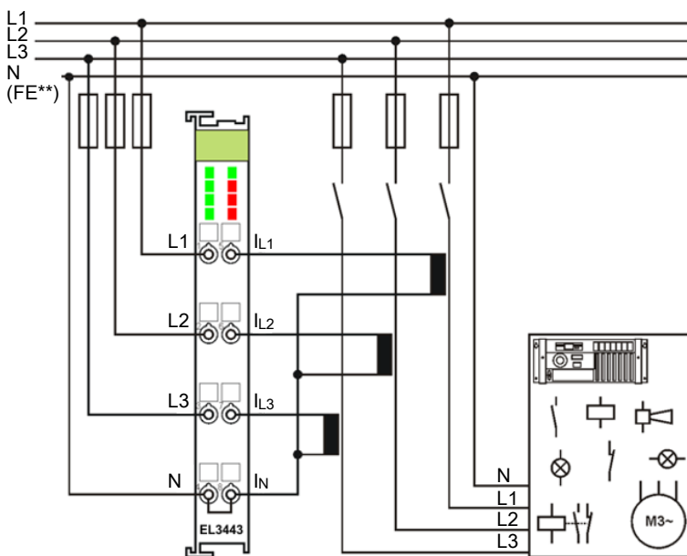
Fig. 40: EL3443, power measurement at a machine
