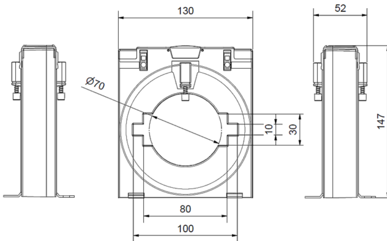
Fig. 28: Right side view, front view, left side view; all dimensions in mm
