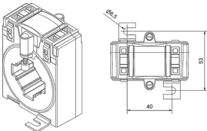
Fig. 19: Isometric view, top view; all dimensions in mm
