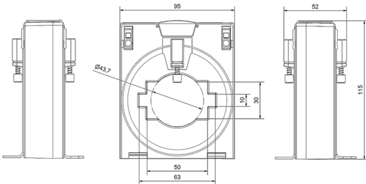
Fig. 24: Right side view, front view, left side view; all dimensions in mm
