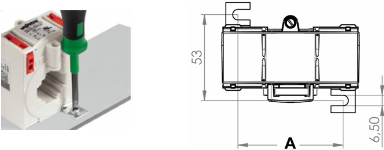
Fig. 35: Mounting on mounting plate
