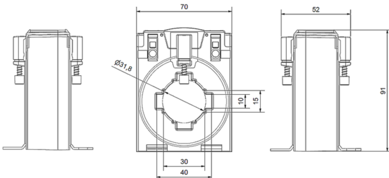
Fig. 20: Right side view, front view, left side view; all dimensions in mm
