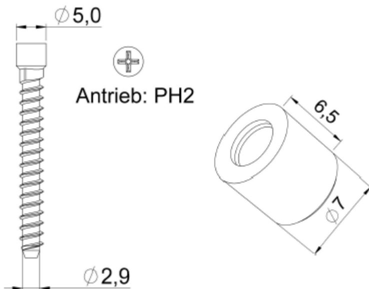
Fig. 27: Tightening torque of fastening screw: 0.5 Nm
