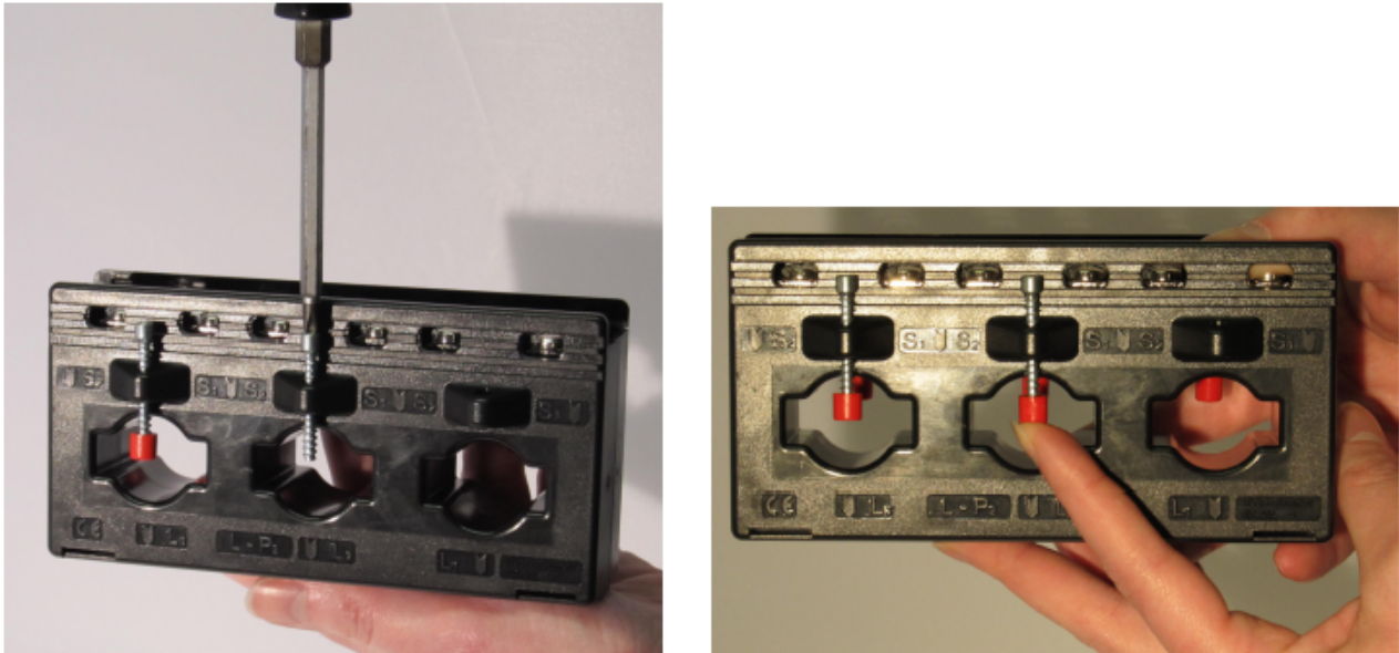
Fig. 25: Mounting the fastening screws SCT3215 , SCT3315
