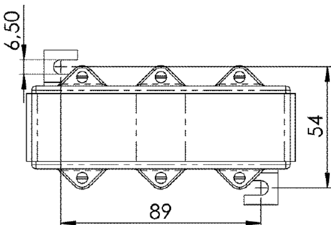
Fig. 28: Mounting on mounting plate SCT3211
