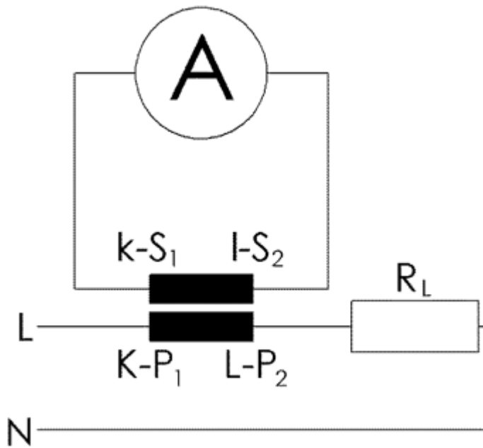
Fig. 23: Measuring circuit - SCT3xxx transformer
