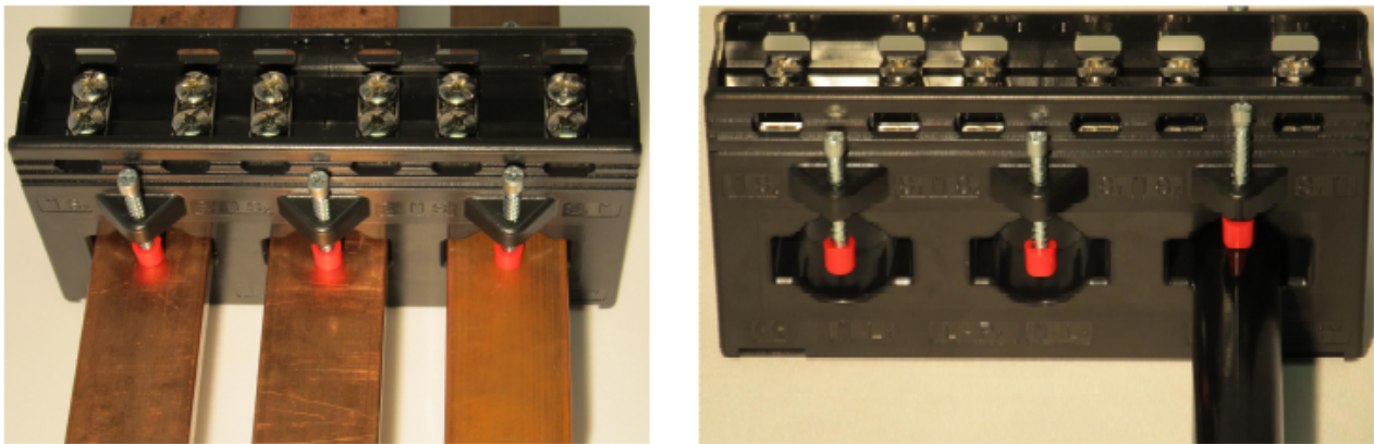
Fig. 26: Mounting on copper bar or round conductor, SCT3215 , SCT3315
