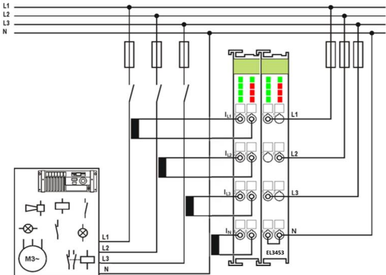
Fig. 32: EL3453, power measurement at a machine
