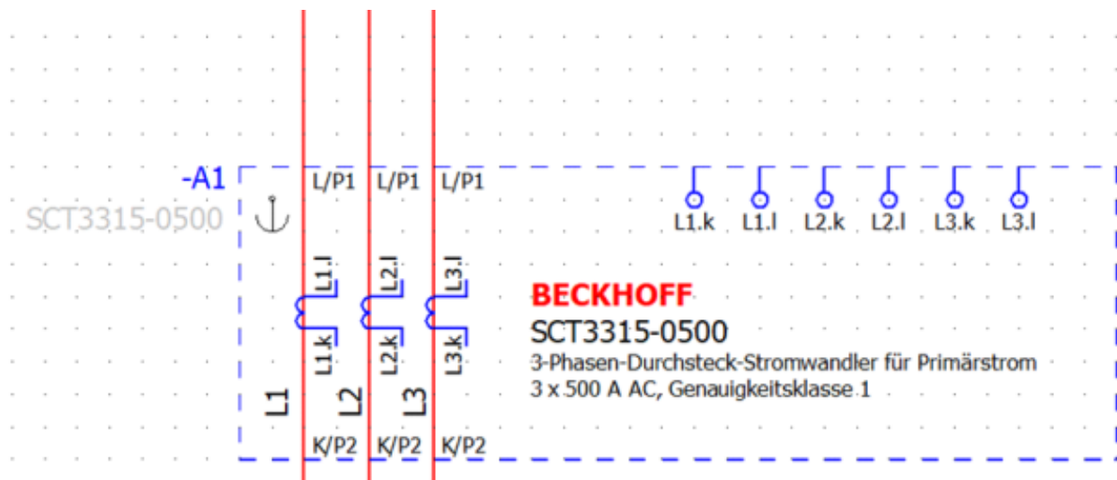
Fig. 24: Example Eplan macro for SCT3xxx current transformers
