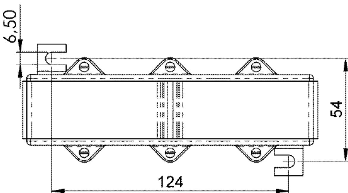
Fig. 29: Mounting on mounting plate SCT3315
