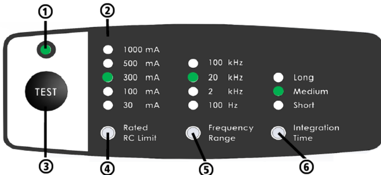
Fig. 25: User interface with input and test button
