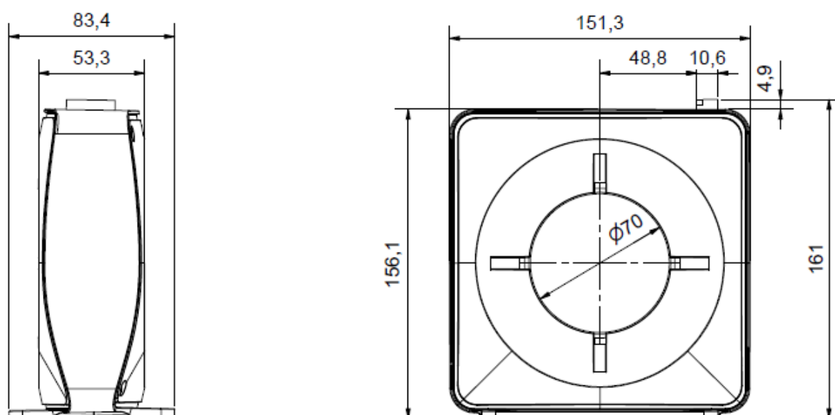
Fig. 17: Side view, front view, all dimensions in mm
