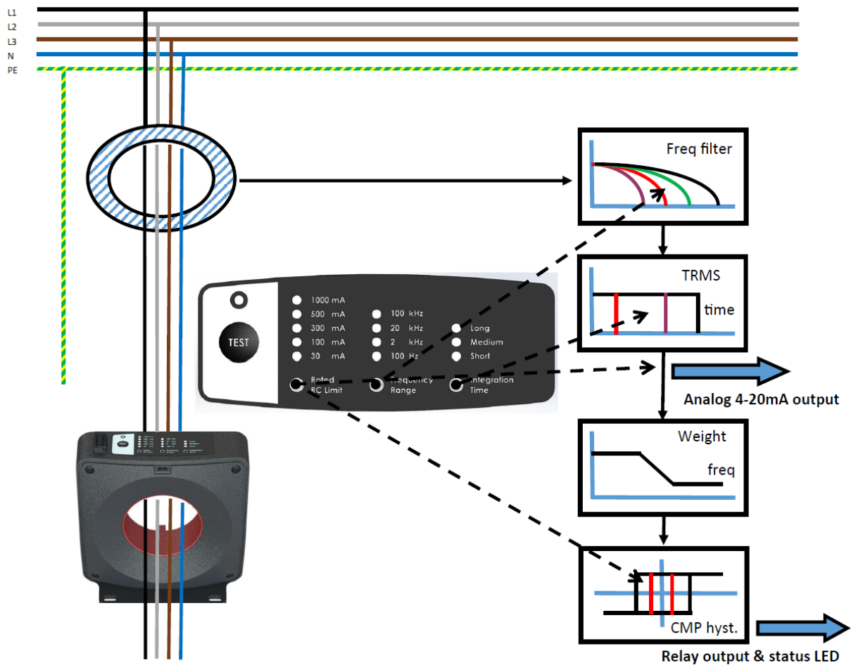
Fig. 23: SCT5xxx block diagram
