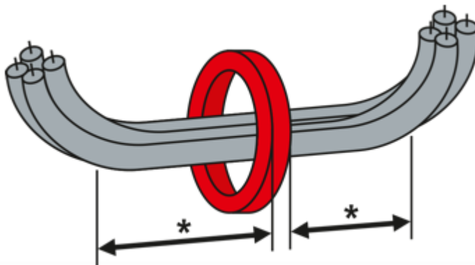
Fig. 19: Calculation bending primary conductor: *distance to 90° angle = 2x outer diameter
