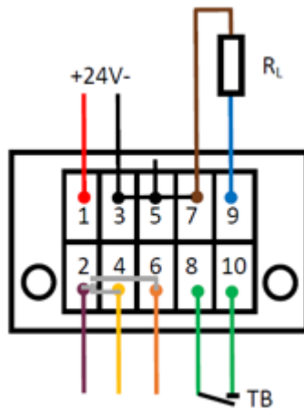
Fig. 22: Connection
