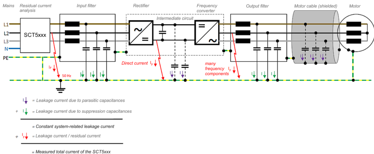
Fig. 27: Electrical equivalent circuit diagram of a speed-controlled motor
